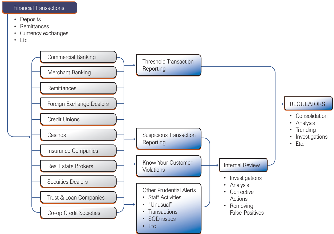
Figure 1 – SymSure for IDEA AML Process Flow
